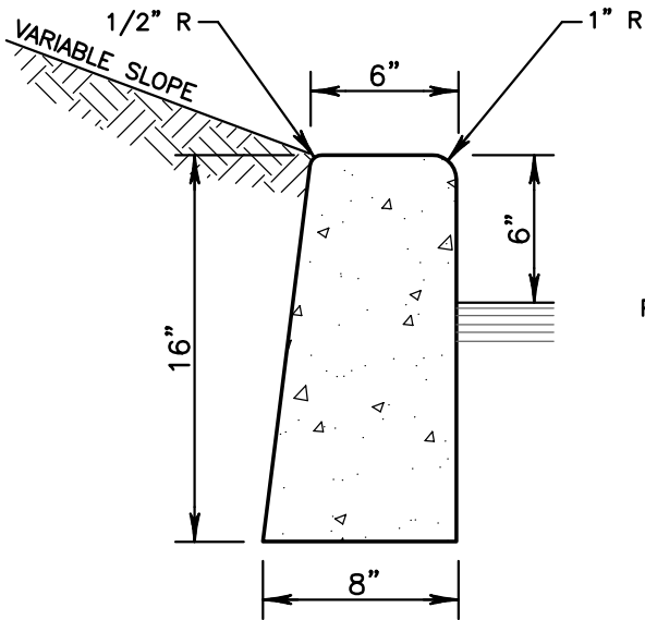
TYPE E-1 CURB
