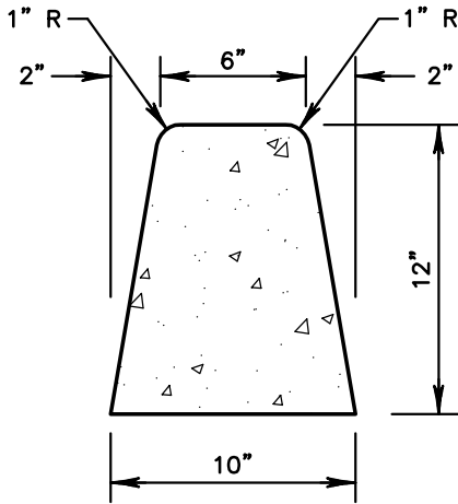
TYPE E-1 CURB
