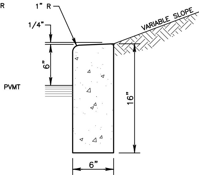
TYPE E-2 CURB
