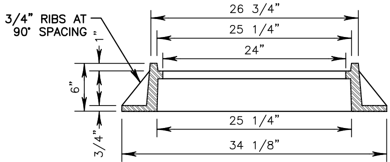
CIRCULAR FRAME
