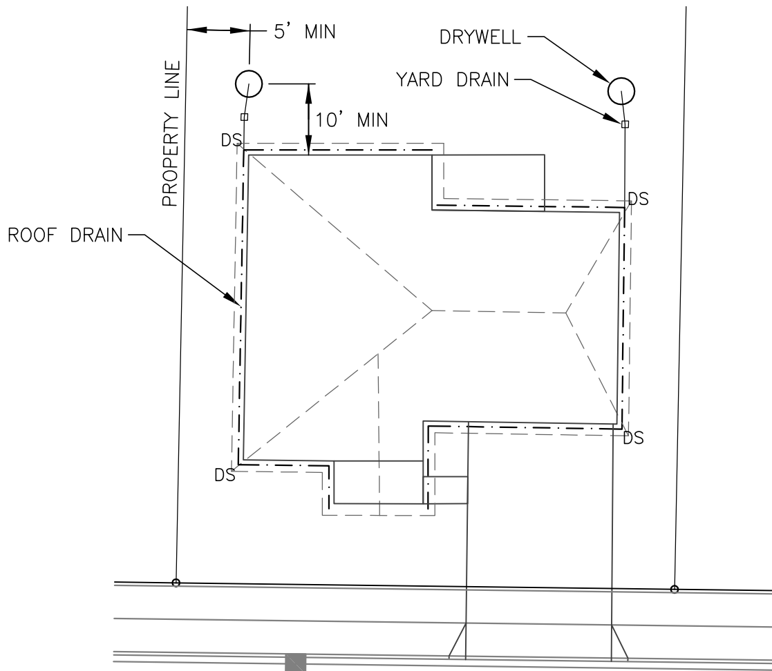
PLAN VIEW
