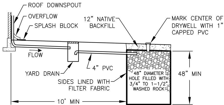
DRYWELL PROFILE
