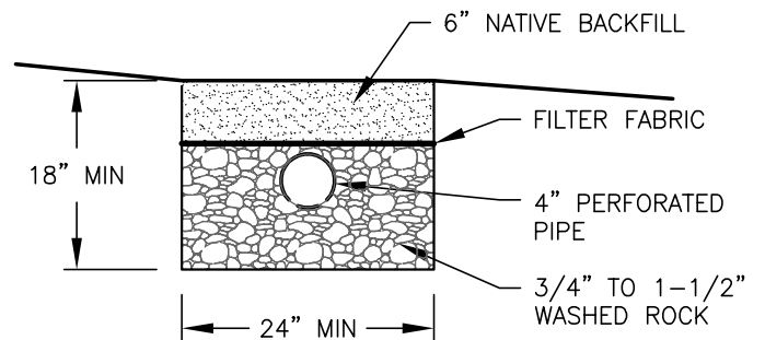
TRENCH SECTION
