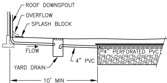
TRENCH PROFILE
